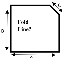
4 Cut Corner
